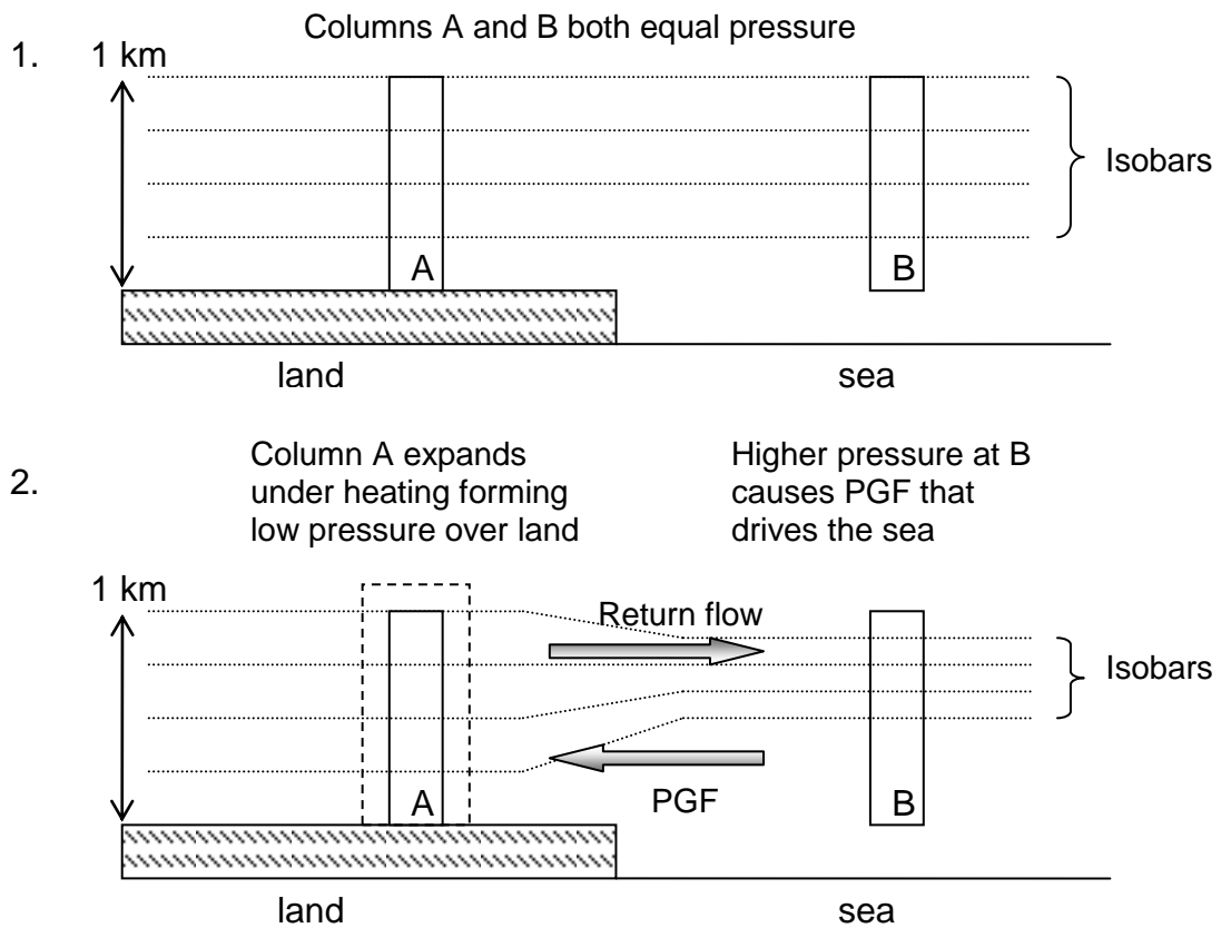
Fig. 2.1. Sea breeze formation under calm conditions. Adapted from Simpson, (1994)
