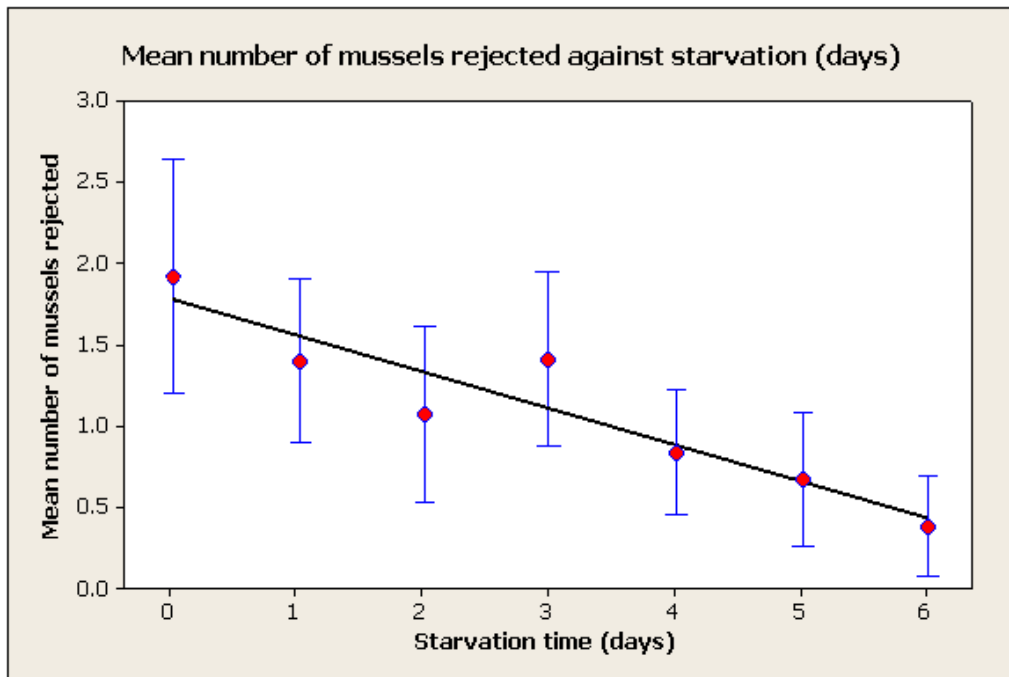
Fig. 5- The mean number of mussels rejected with increased starvation time. Linear regression line (Equation- No. of mussels rejected = 1.777 - 0.2232 Ts) showing a negative correlation. Confidence intervals included (95%)
