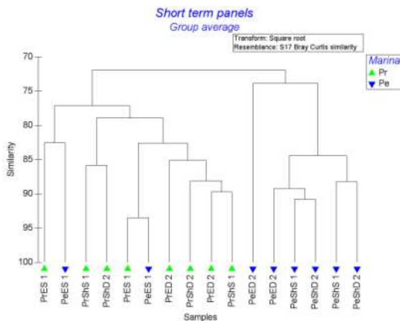
Figure 15. Premier and Port Pendennis Marina. Dendrogram of hierarchical clustering of 16 sites, using group average linking of Bray Curtis similarities calculated on \sqrt{\text{transformed}} abundance data. The different sites within marinas are as follows; PR – Premier, PE – Pendennis, Sh – Sheltered, E – Exposed, S – surface, D – Deep.
