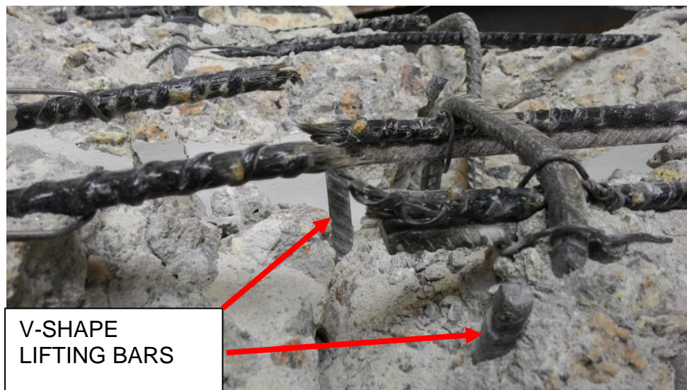
Photo 13: Beam B4 Reinforcement Failure.
