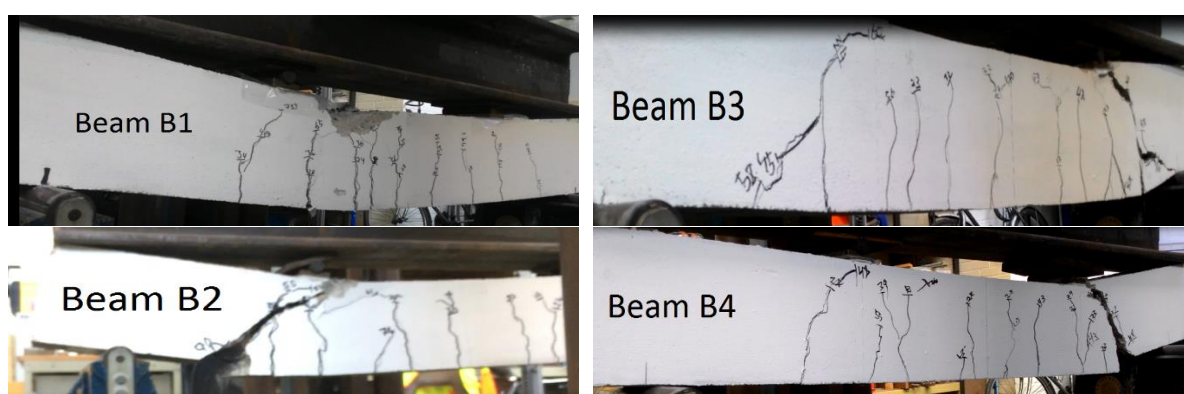
Photo 6: Failure Modes of Each Beam.
