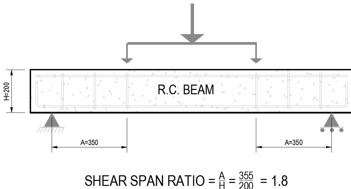
Figure 7: Shear Span Ratio of the Reinforced Concrete Beams.
