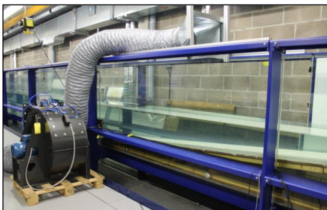
Figure 11: Wind generator set up
