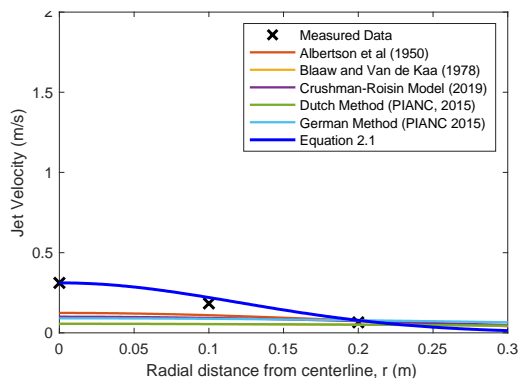
Figure 23: Comparative radial velocity decay graph at x=2.5\text{m}
