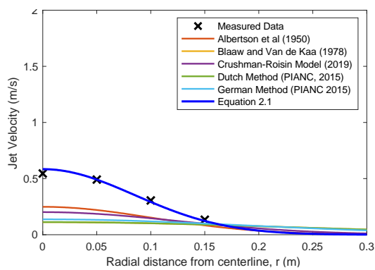
Figure 20: Comparative radial velocity decay graph at x=1.25\text{m}
