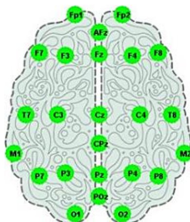
Figure 1: Layout of Electrodes in the 10-20 EEG System.
