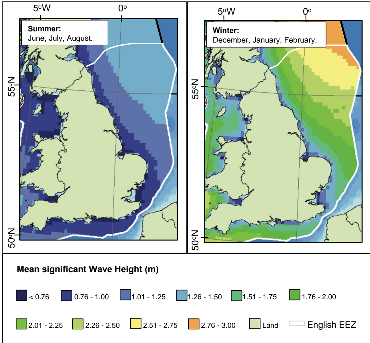
Figure 7: Annual extremes in the seasonal mean significant wave height across the UK's exclusive economic zone. Modelled wave data is less robust in shallow waters (<20m) and zones of complex bathymetry. Wave data is based on hourly values from 2000 – 2007. This figure (modified from ABPmer, 2008) has been used to illustrate wave heights: Reproduced from http://www.renewables-atlas.info /© Crown Copyright.
