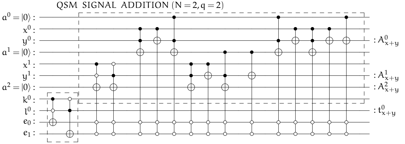
Figure 2.16: QSM signal addition operation (2-qubit long, 2-qubit amplitude depth).
