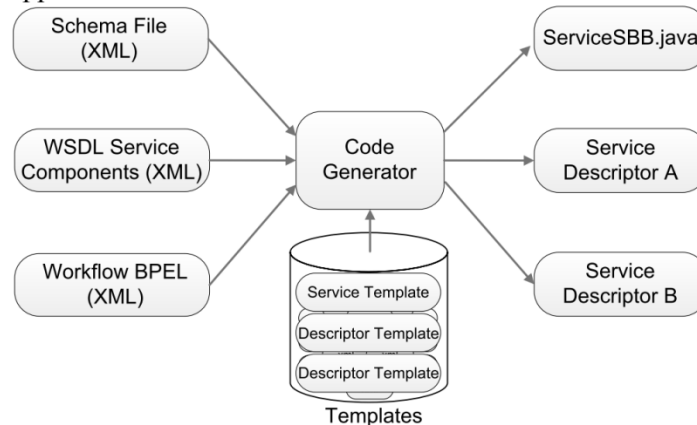
Figure 2: CodeGenerator
