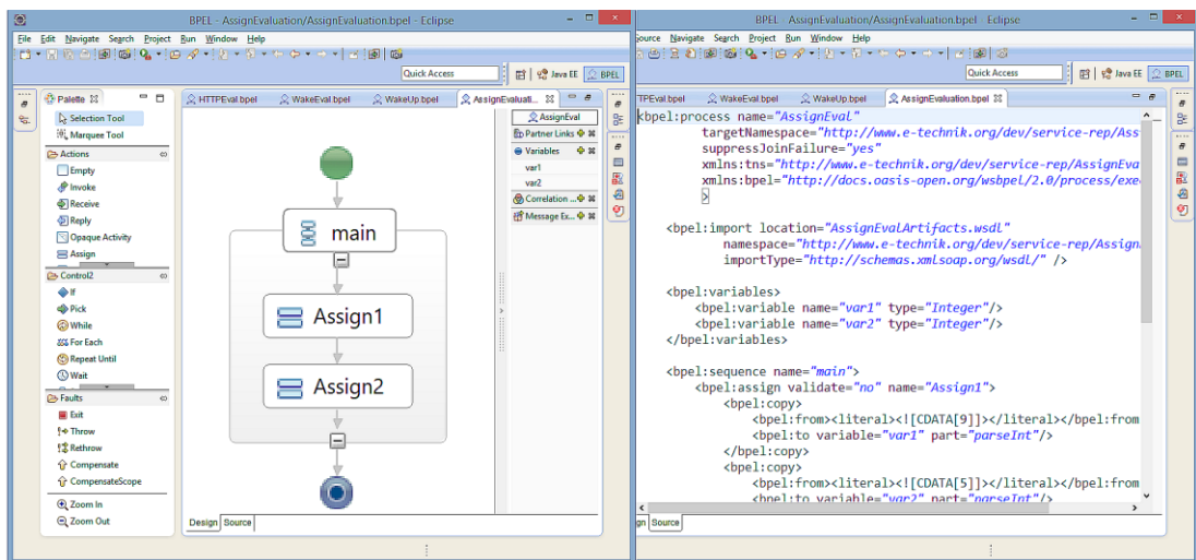
Figure 8.2: Eclipse BPEL developer
