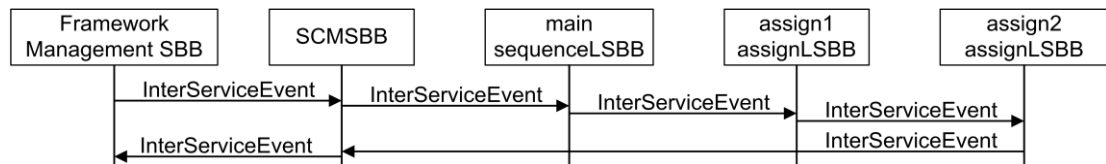
Figure 8.29: Assign execution phase MSC
