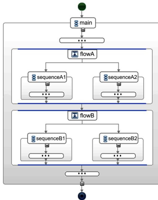
Figure 5.14: BPEL process with two flow activities within a sequence and the resulting SBBs
